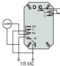
Normally Closed
